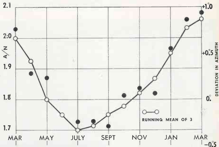
Top chart shows monthly variation of A/N of air beacon, obscured at 10-mile distance. Other charts show sharp shifts in bearings during rain and snow falls.
