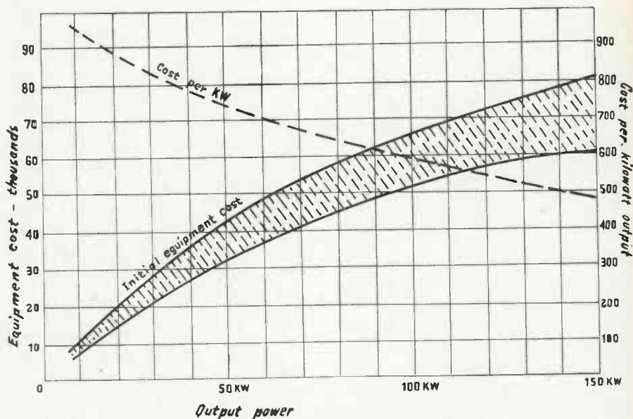
Initial cost of radio-frequency equipment and cost per kw based on a number of installations made by different manufacturers
