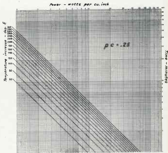
Same as chart at left, except for wood or other material having a value of pc = .25
