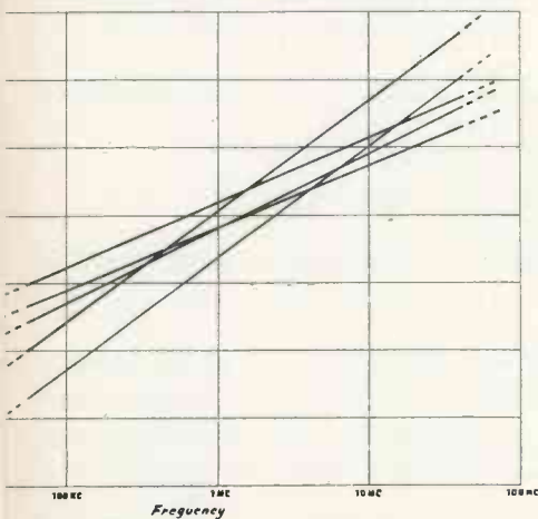
Variation of power factor with frequency. At higher frequencies these curves tend to flatten out
