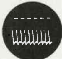
Oscillogram showing the precise wave form of the DuMont Variable-Frequency Stimulator for brain surgery and research. The remarkable uniformity of wave form and amplitude of the stimuli, is clearly disclosed here. Time interval: 1 millisecond.
