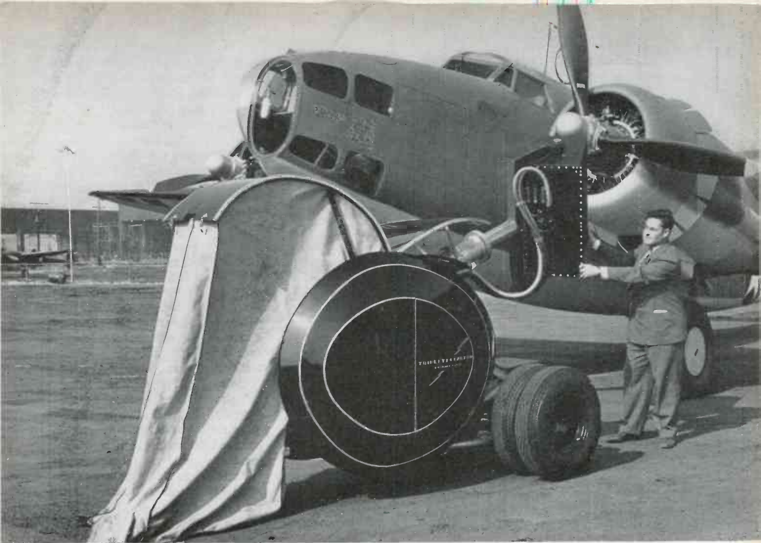
Mobile 250 kv X-ray unit with own darkroom for front-line radiographing of aircraft, demonstrated by designer Tom Triplett
