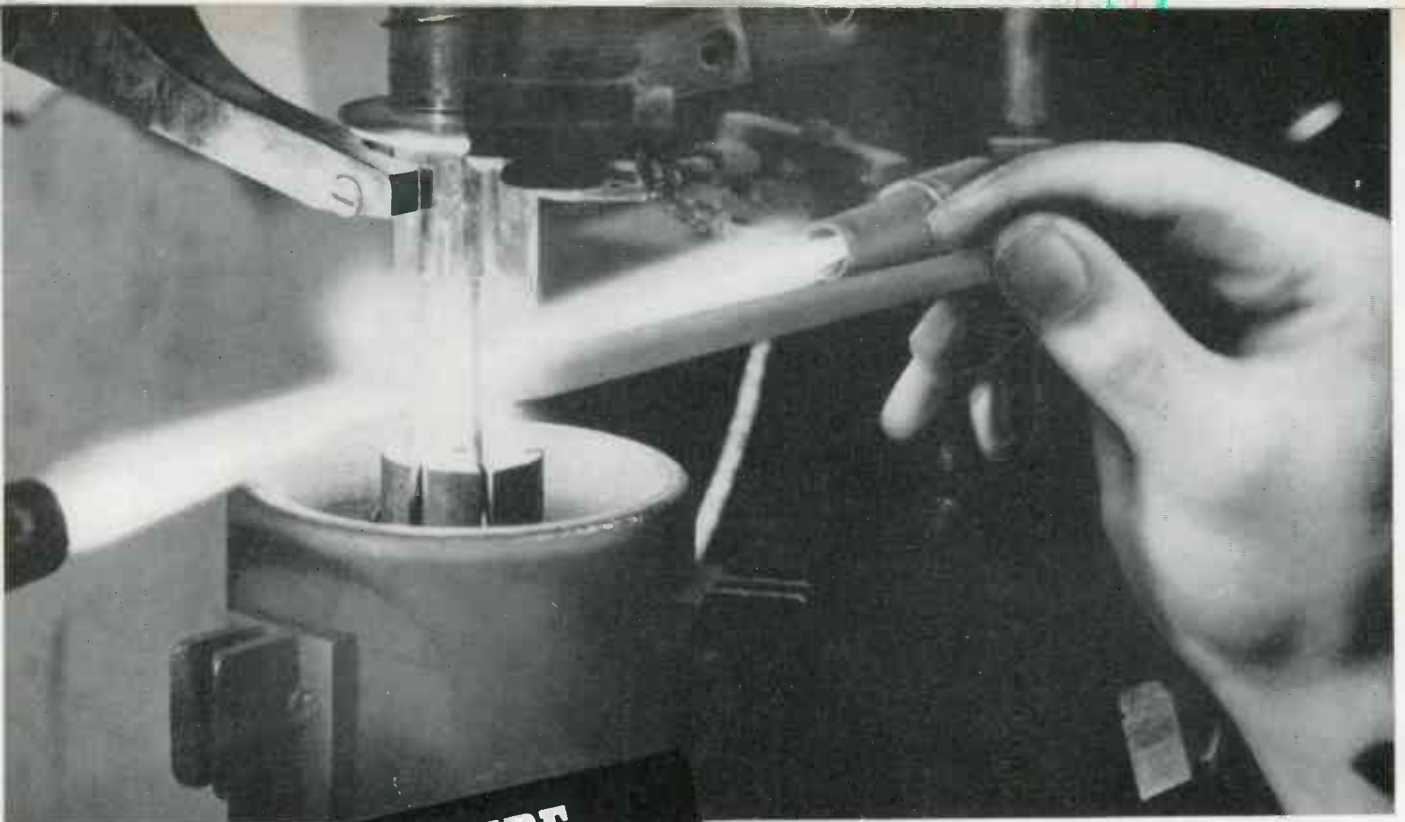
Glass tubing becomes finished filament stem with leads sealed in position on this special upright lathe.
