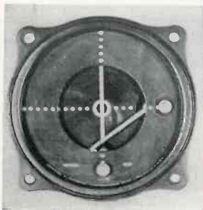
↑ Cross-pointer indicator
