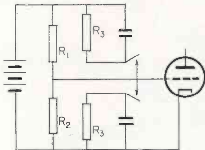
Exponential resistor
