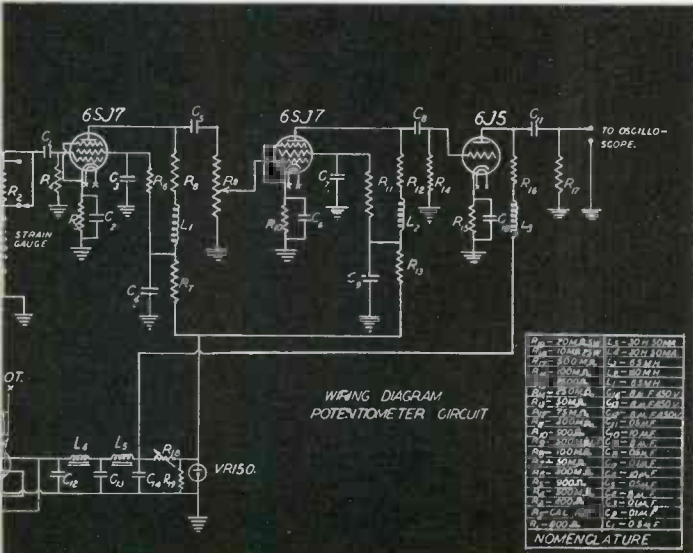
Amplifier for cycle vibration study with strain gage as arm of potentiometer
