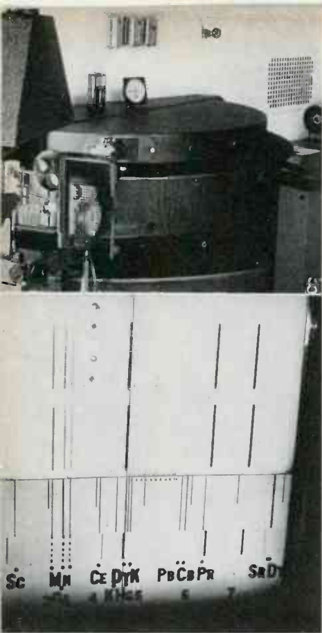
Materials analysis by visual (qualitative) and photoelectric (quantitative) examination of spectrograms obtained with this equipment speed aircraft engine production. At top, apparatus for photographing spectrum of vaporized sample. Below, checking projected image of spectrum against master scale
