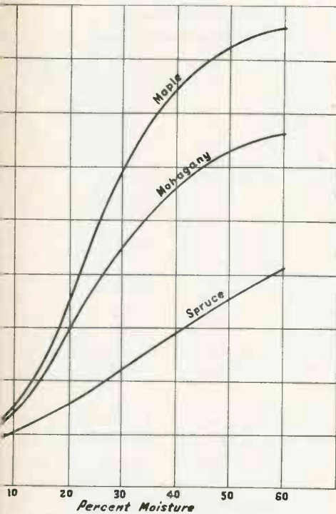
Variation of power factor with per cent moisture for three woods. Curves should be used only as a first approximation
