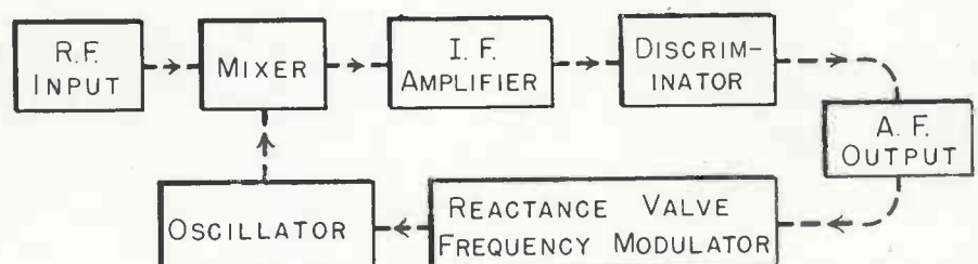
Frequency-following superheterodyne receiver
