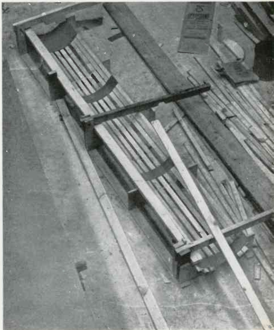
Studio panels of WSPD, Toledo, during construction. Compo board is bent on forms of the required curvature
