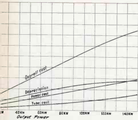
Approximate tube, power and overall operating cost versus power delivered to the load
